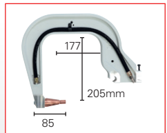
C3 Arm (CEL019157) Insulated C3 (CEL021419)
