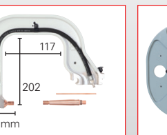
C8 Arm (CEL020016) Insulated C8 (CEL021440)
