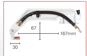
C5 Arm (CEL019294) Insulated C5 (CEL022393)
